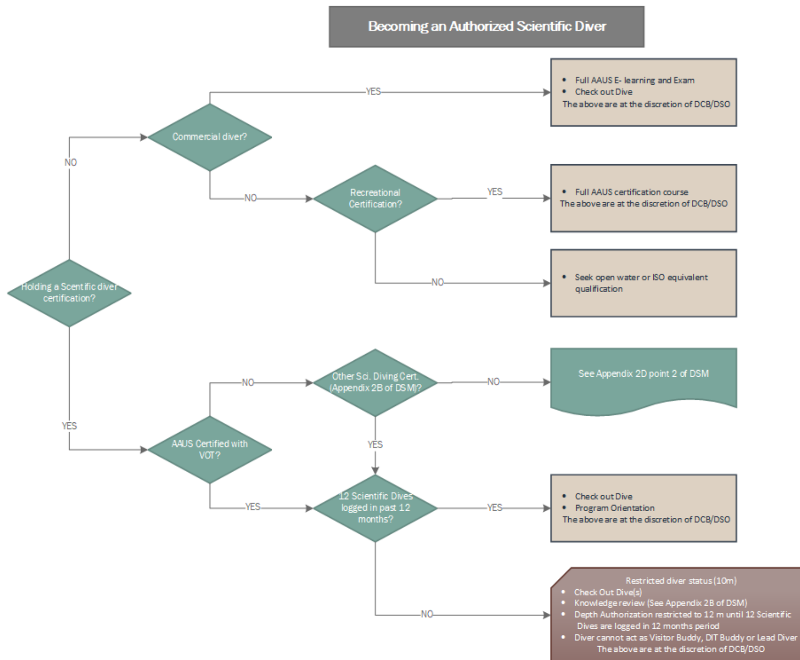
Figure 1 - Flowchart 1
