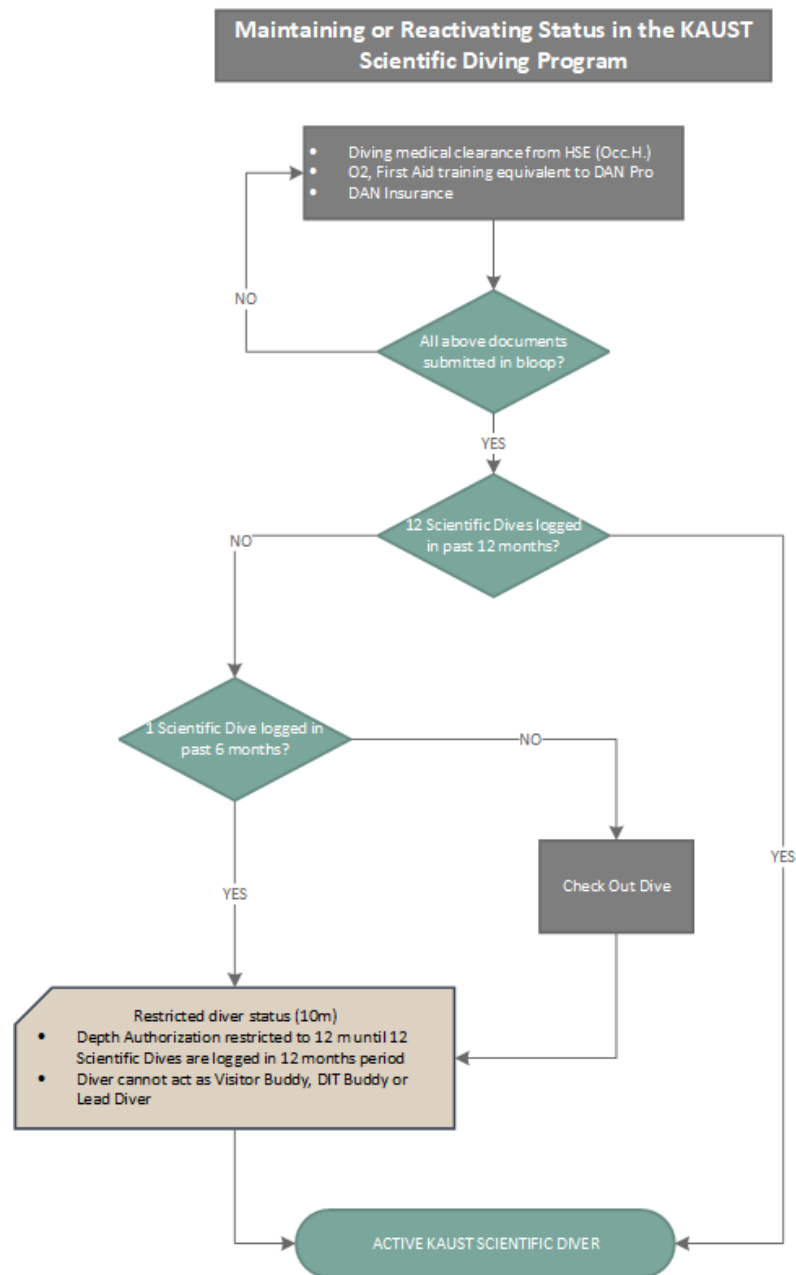
Figure 2 - Flowchart 2
